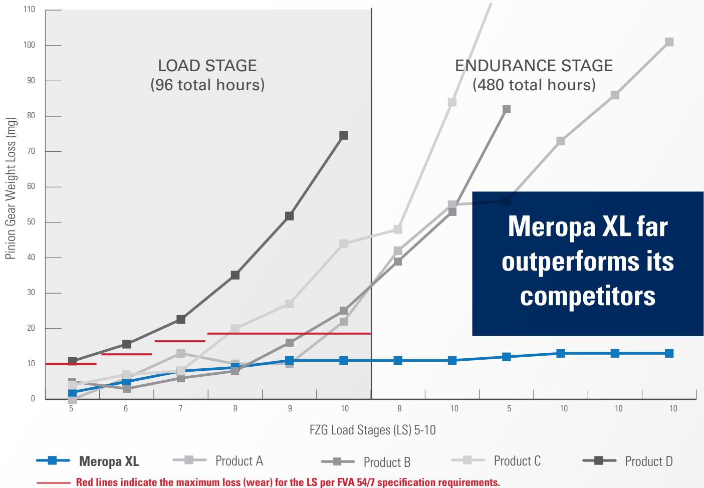
FVA 54/7 Pinion Gear Weight Loss
